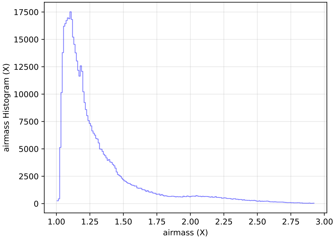
ddf_acor_sf15_lsf20_lsr50_v3.4_10yrs WFD i band: airmass Histogram
