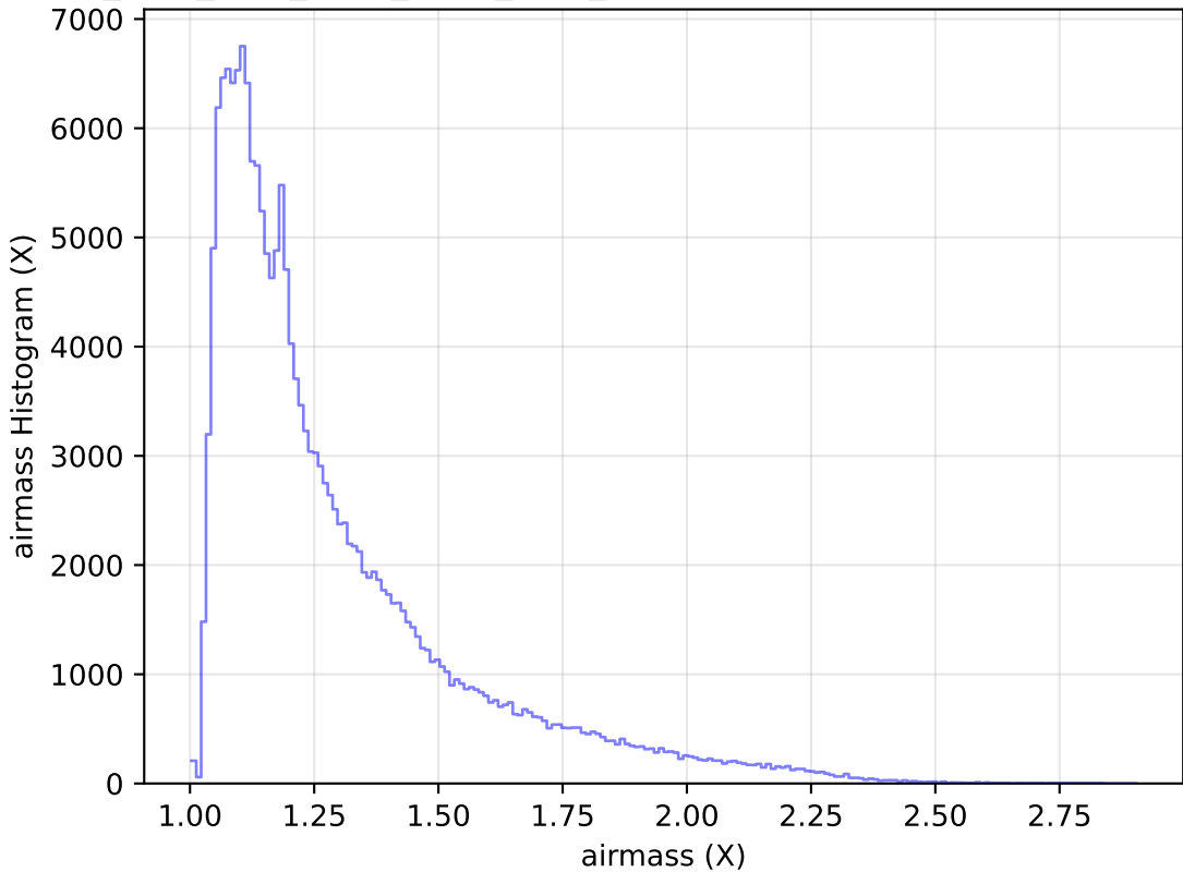
ddf_acor_sf15_lsf20_lsr50_v3.4_10yrs WFD g band: airmass Histogram
