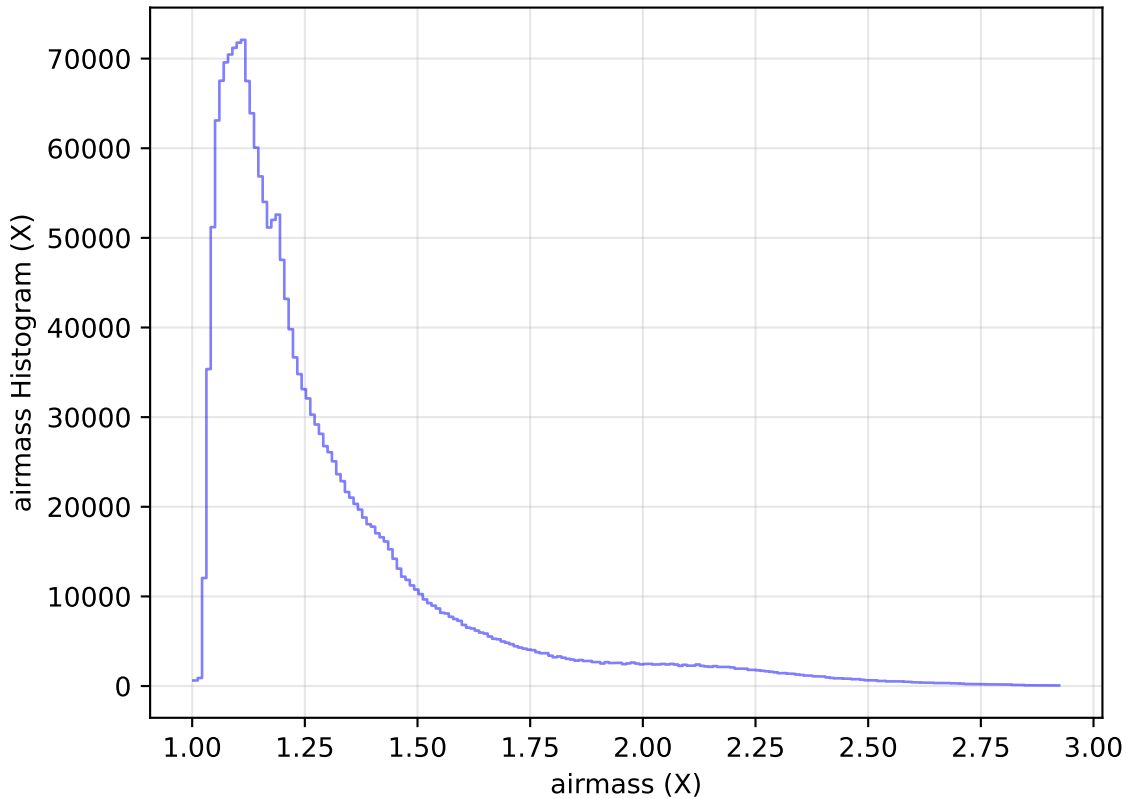
ddf_acor_sf15_lsf20_lsr50_v3.4_10yrs WFD all bands: airmass Histogram
