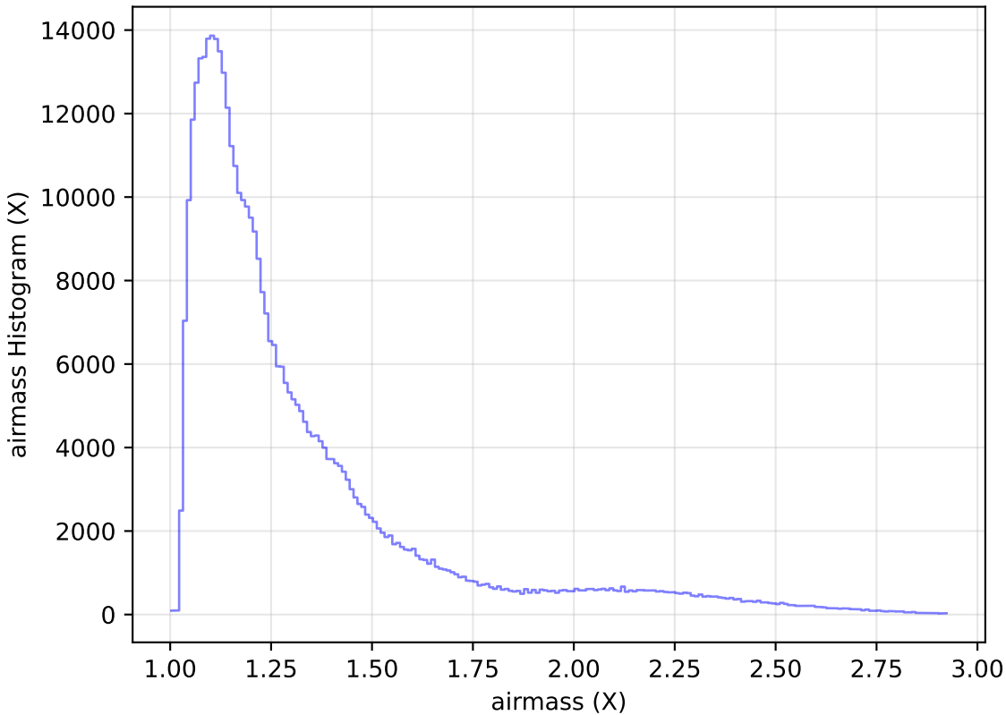
ddf_acor_sf15_lsf20_lsr50_v3.4_10yrs All sky z band: airmass Histogram
