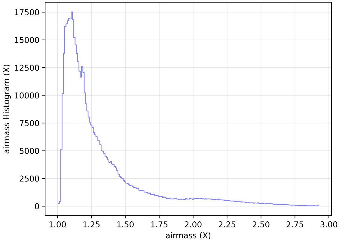
ddf_acor_sf15_lsf20_lsr50_v3.4_10yrs All sky i band: airmass Histogram
