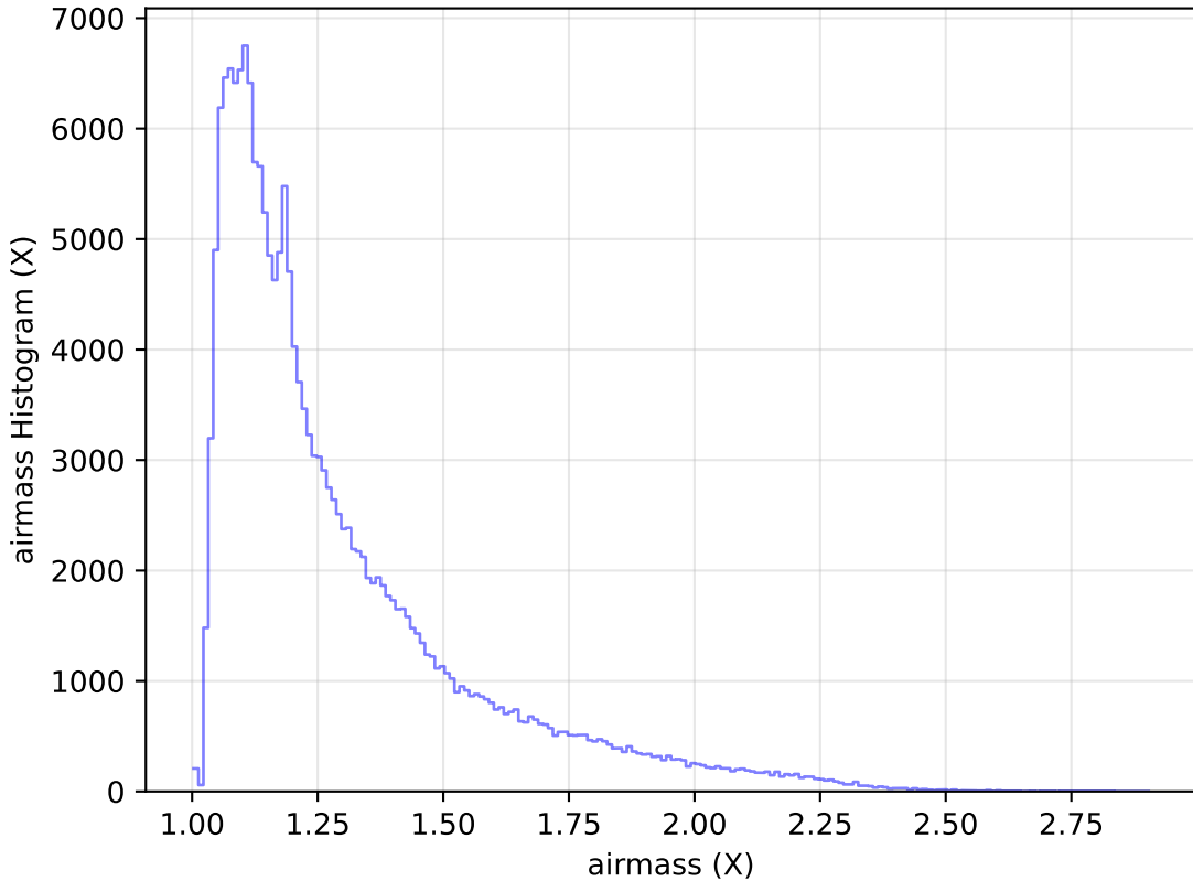
ddf_acor_sf15_lsf20_lsr50_v3.4_10yrs All sky g band: airmass Histogram
