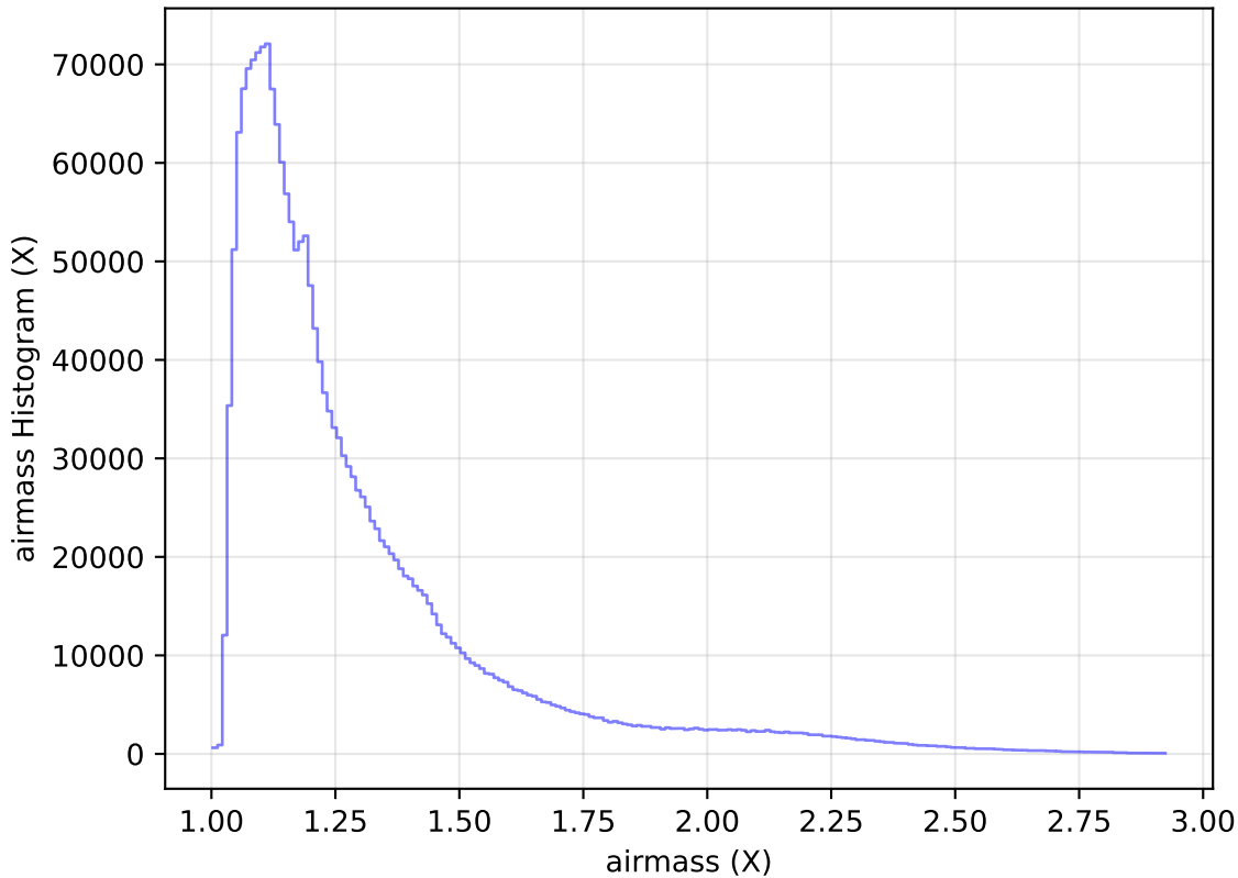
ddf_acor_sf15_lsf20_lsr50_v3.4_10yrs All sky all bands: airmass Histogram
