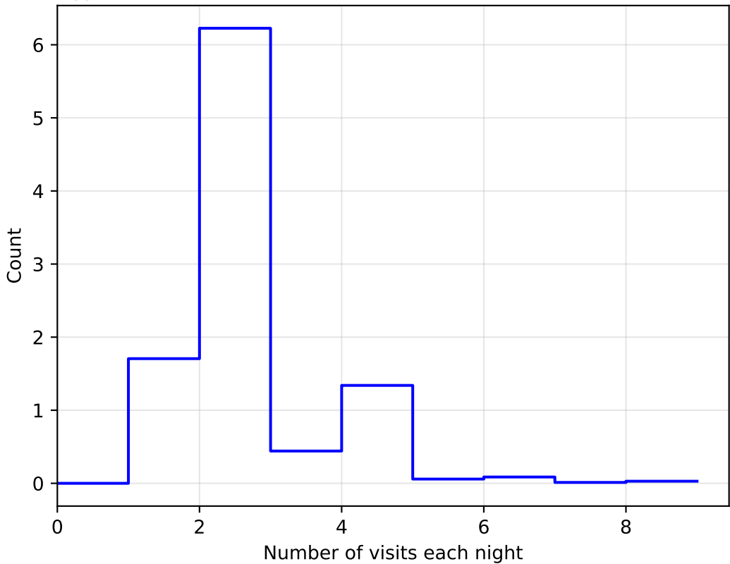
ddf_acor_sf15_lsf20_lsr50_v3.4_10yrs All sky: NVisitsPerNight 1e6
