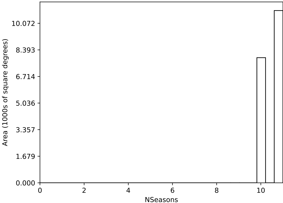
ddf_acor_sf15_lsf20_lsr50_v3.4_10yrs WFD all bands: NSeasons
