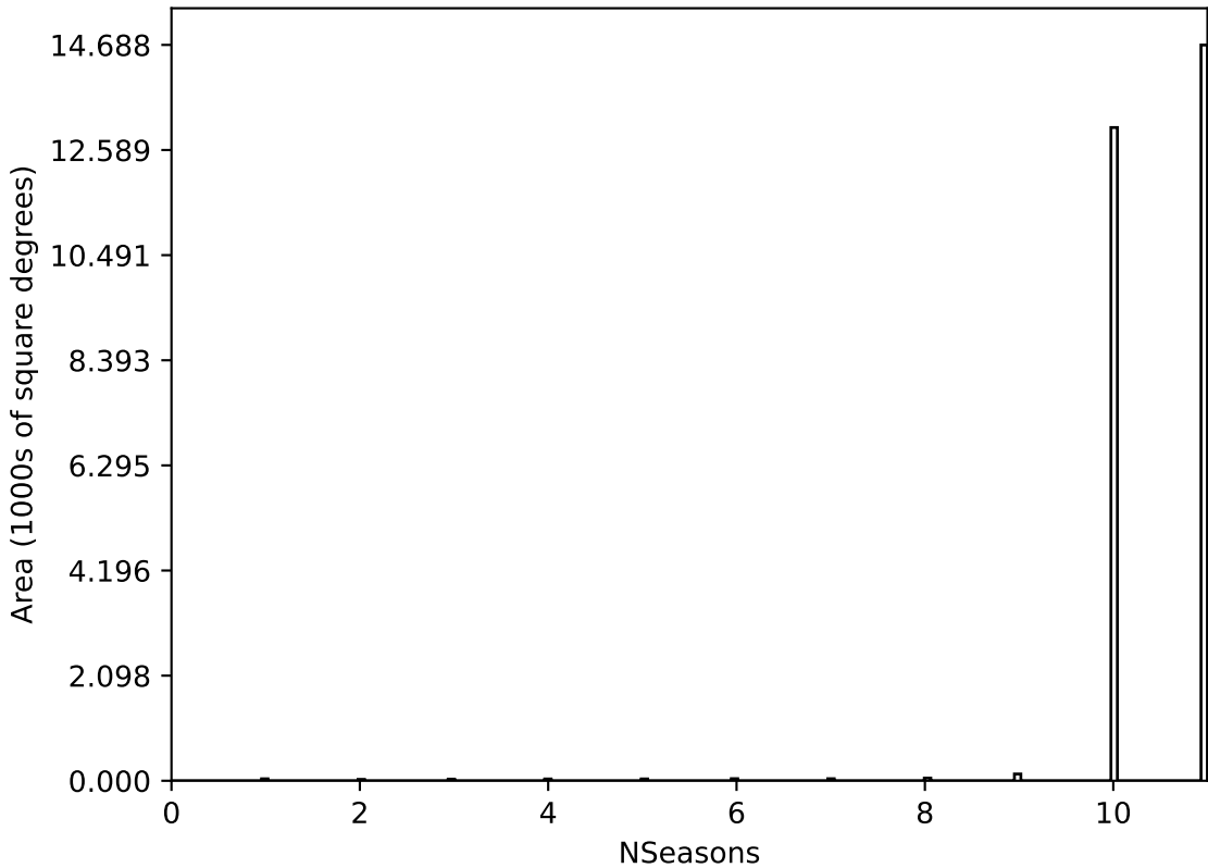
ddf_acor_sf15_lsf20_lsr50_v3.4_10yrs All sky all bands: NSeasons
