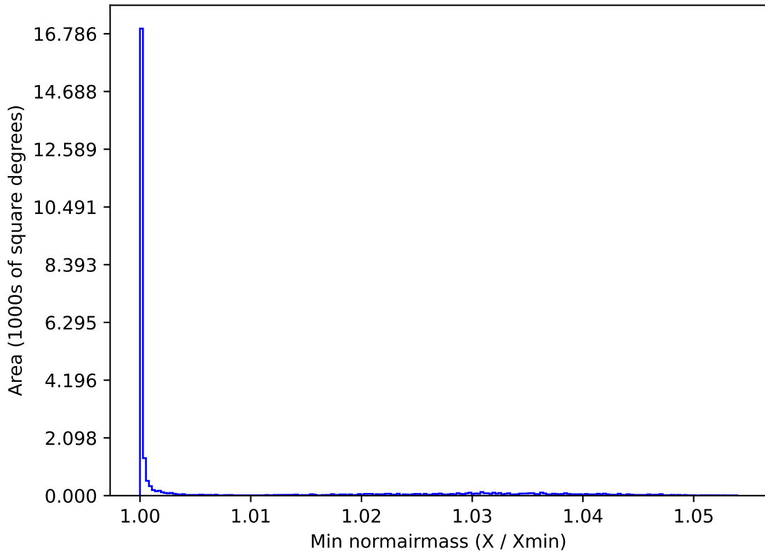
ddf_acor_sf15_lsf20_lsr50_v3.4_10yrs All sky g band: Min normairmass
