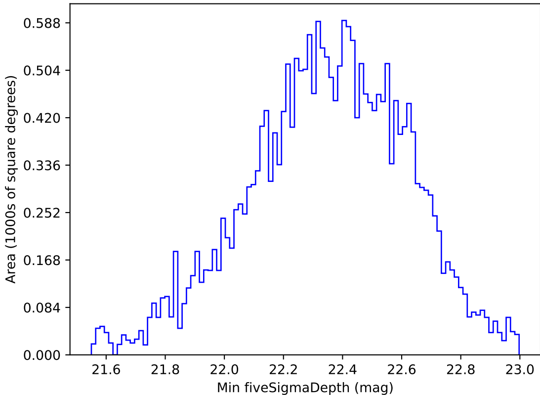
ddf_acor_sf15_lsf20_lsr50_v3.4_10yrs All sky u band: Min fiveSigmaDepth
