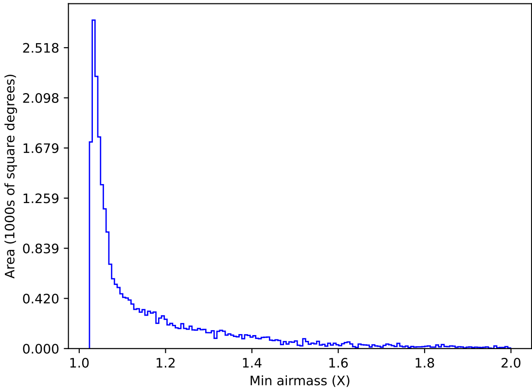
ddf_acor_sf15_lsf20_lsr50_v3.4_10yrs Yr 1 r band: Min airmass
