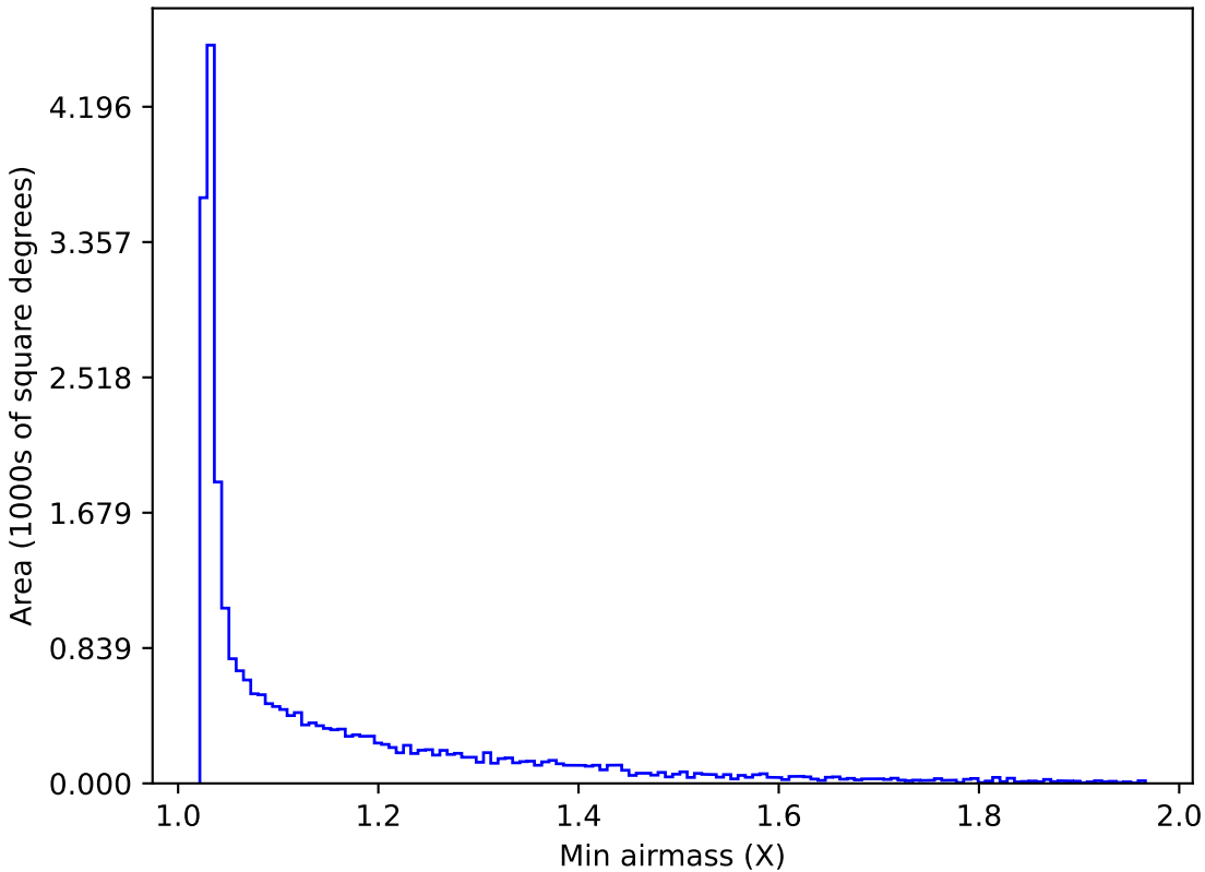
ddf_acor_sf15_lsf20_lsr50_v3.4_10yrs Yr 1 all bands: Min airmass
