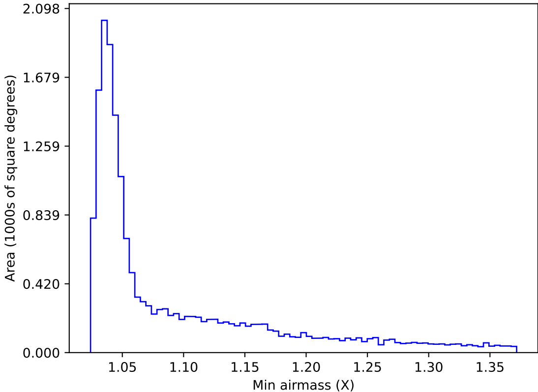
ddf_acor_sf15_lsf20_lsr50_v3.4_10yrs WFD u band: Min airmass
