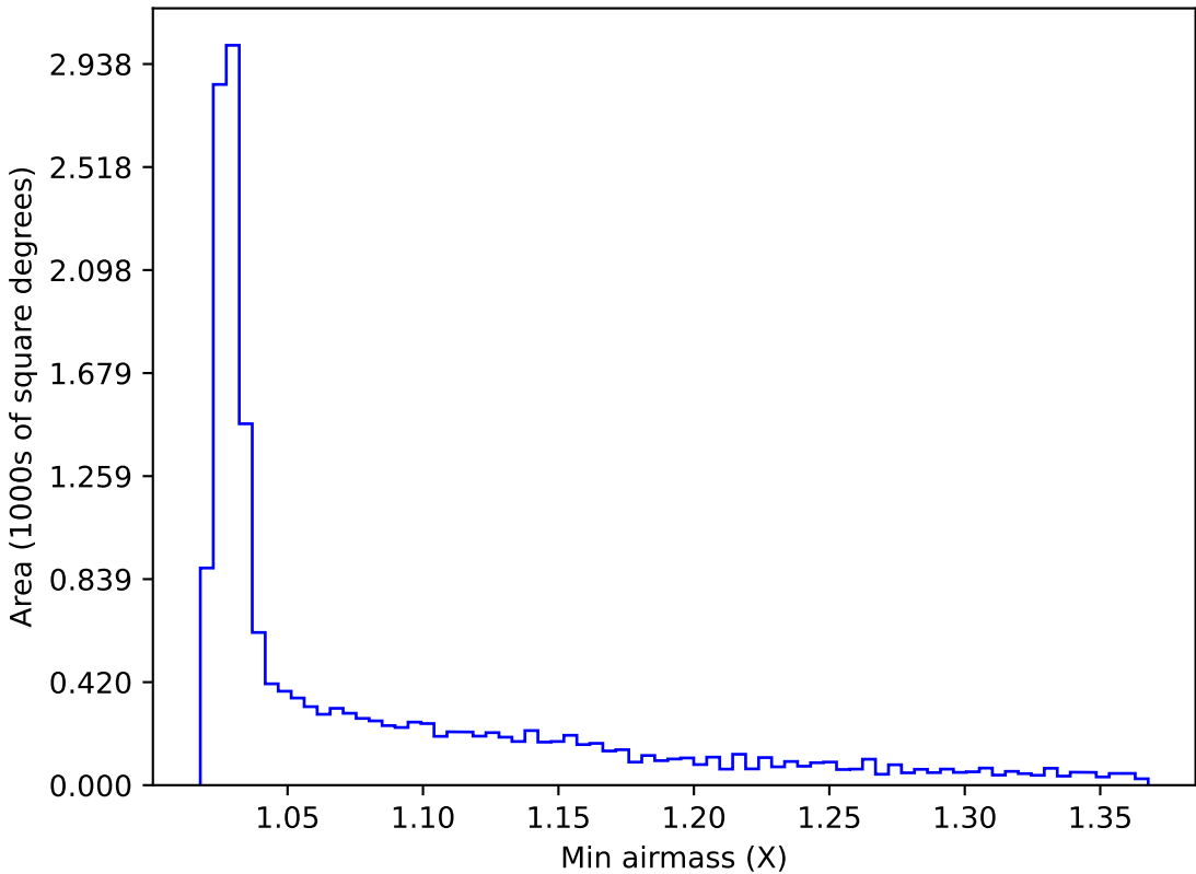
ddf_acor_sf15_lsf20_lsr50_v3.4_10yrs WFD i band: Min airmass
