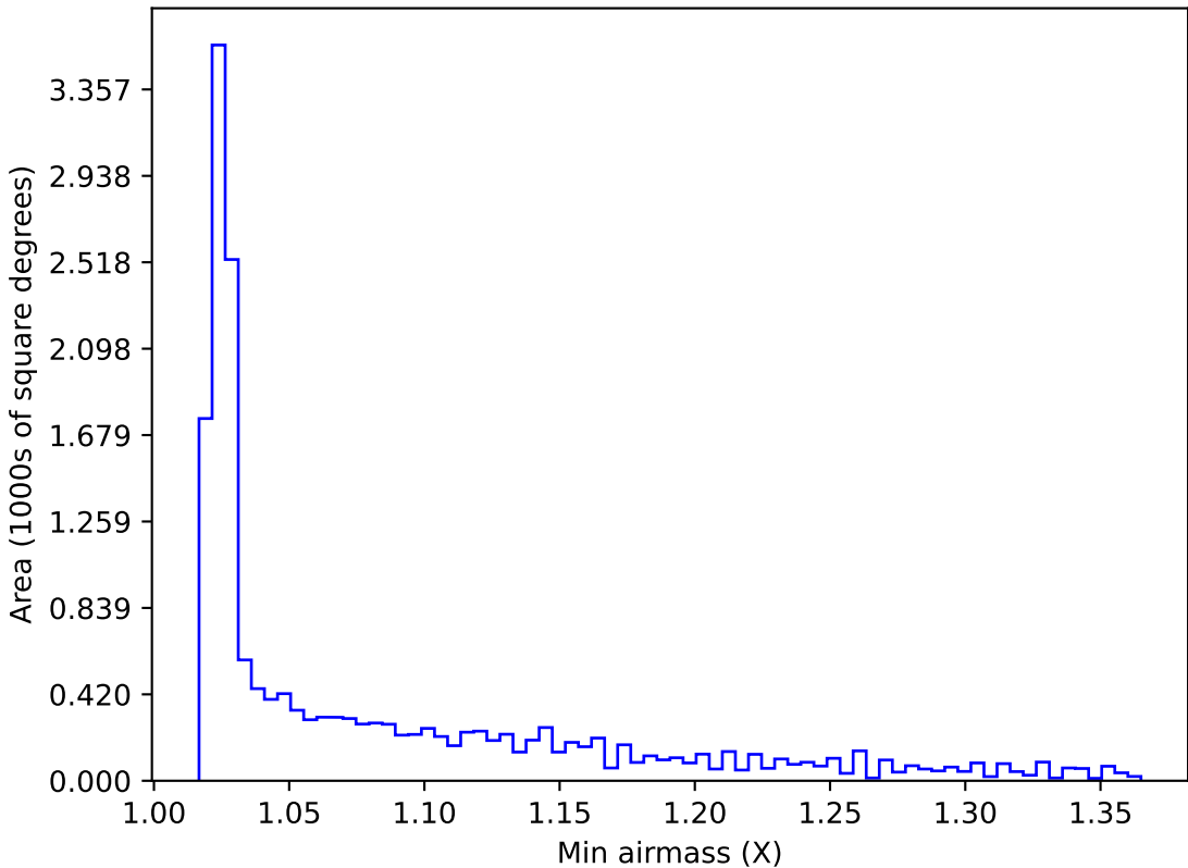
ddf_acor_sf15_lsf20_lsr50_v3.4_10yrs WFD all bands: Min airmass
