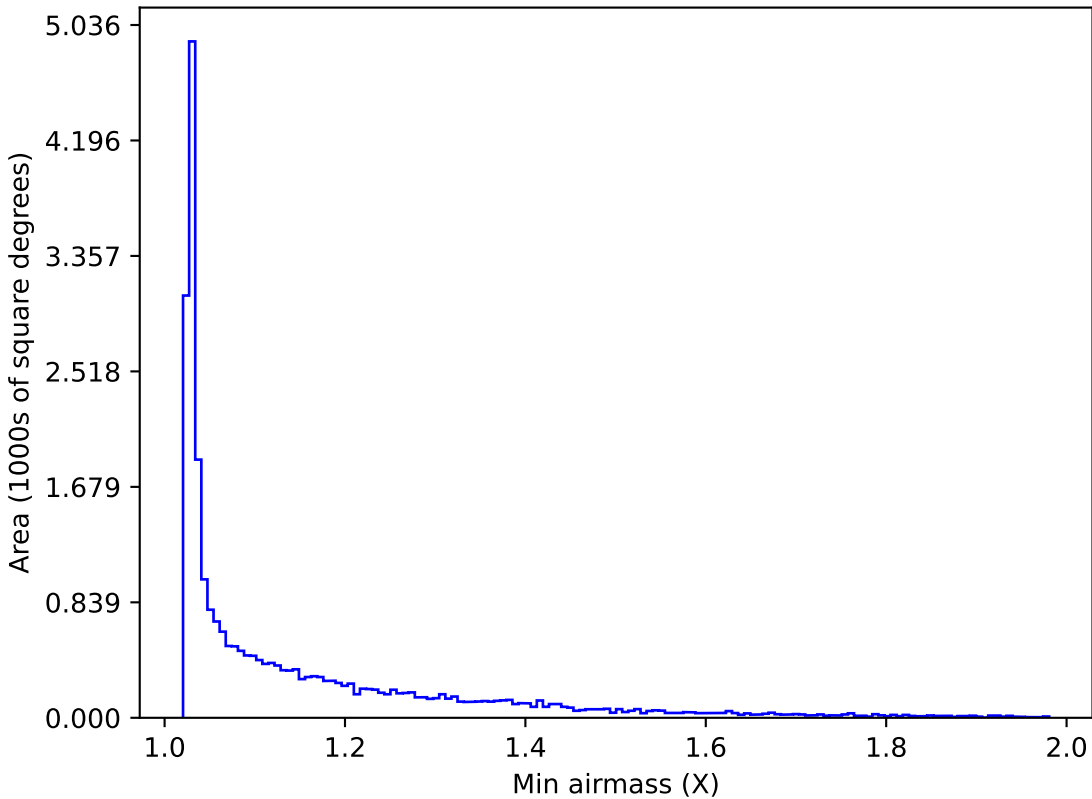
ddf_acor_sf15_lsf20_lsr50_v3.4_10yrs All sky z band: Min airmass
