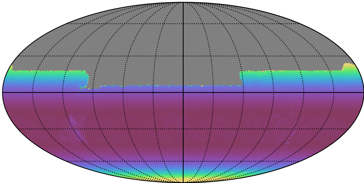
ddf_acor_sf15_lsf20_lsr50_v3.4_10yrs All sky y band: Min airmass
