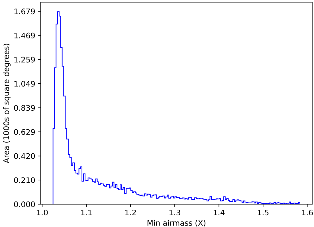
ddf_acor_sf15_lsf20_lsr50_v3.4_10yrs All sky u band: Min airmass
