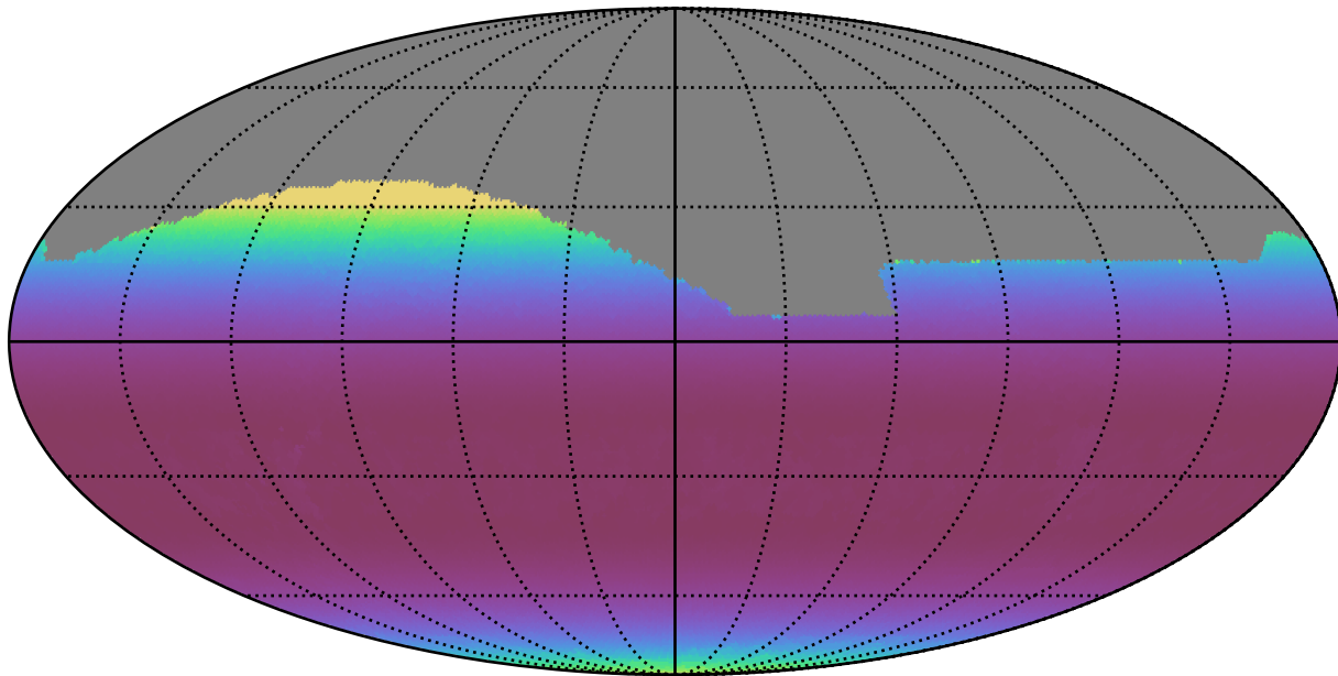
ddf_acor_sf15_lsf20_lsr50_v3.4_10yrs All sky r band: Min airmass
