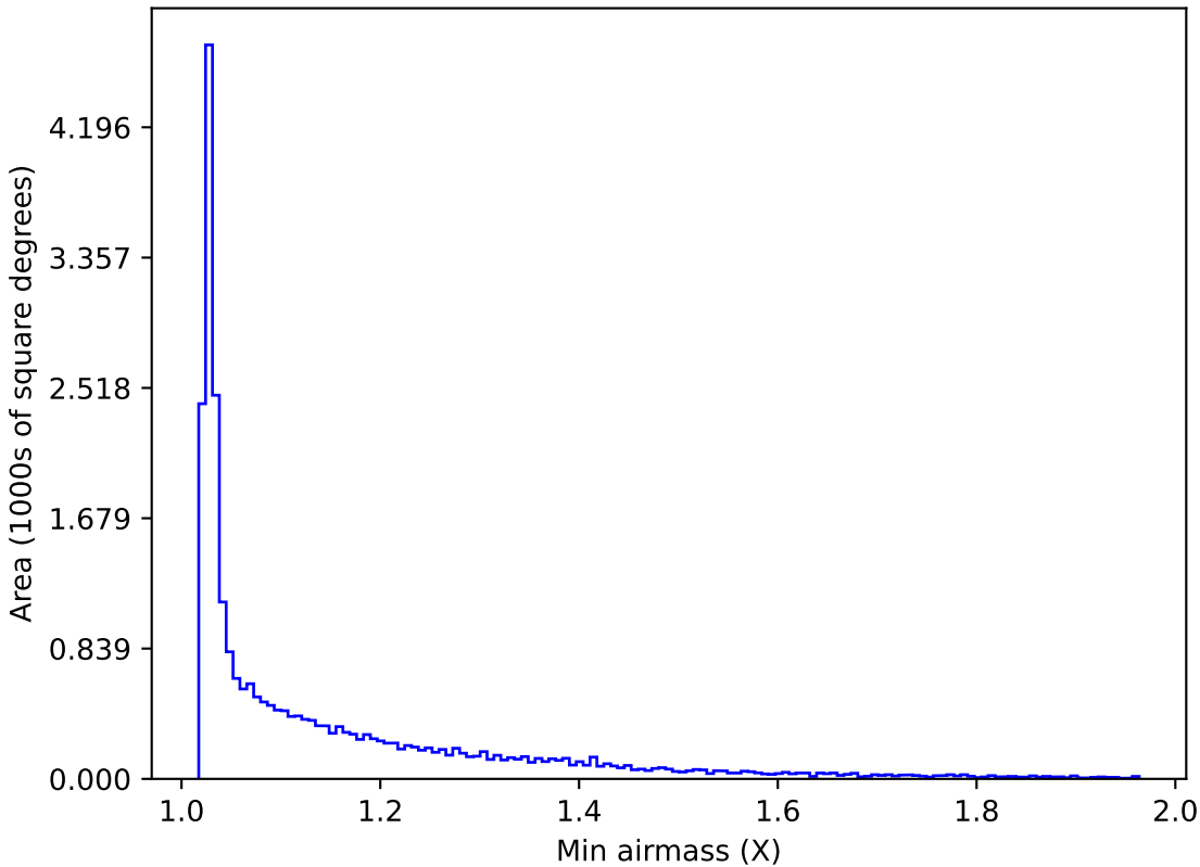
ddf_acor_sf15_lsf20_lsr50_v3.4_10yrs All sky r band: Min airmass
