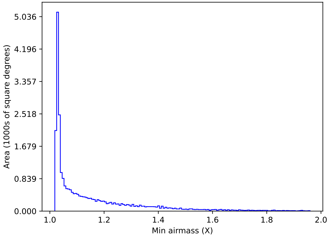
ddf_acor_sf15_lsf20_lsr50_v3.4_10yrs All sky i band: Min airmass
