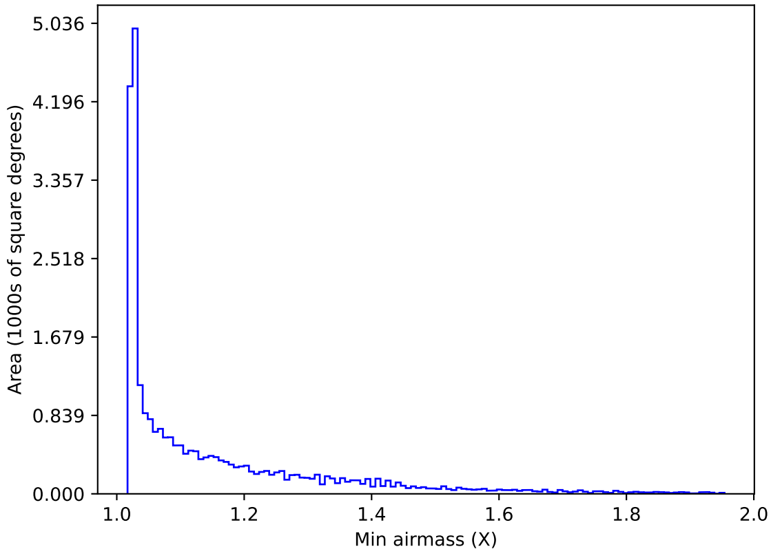
ddf_acor_sf15_lsf20_lsr50_v3.4_10yrs All sky all bands: Min airmass
