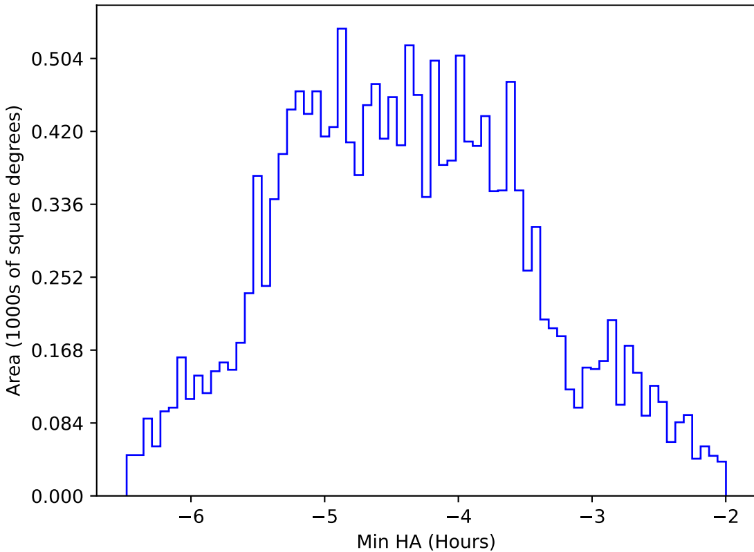
ddf_acor_sf15_lsf20_lsr50_v3.4_10yrs WFD z band: Min HA
