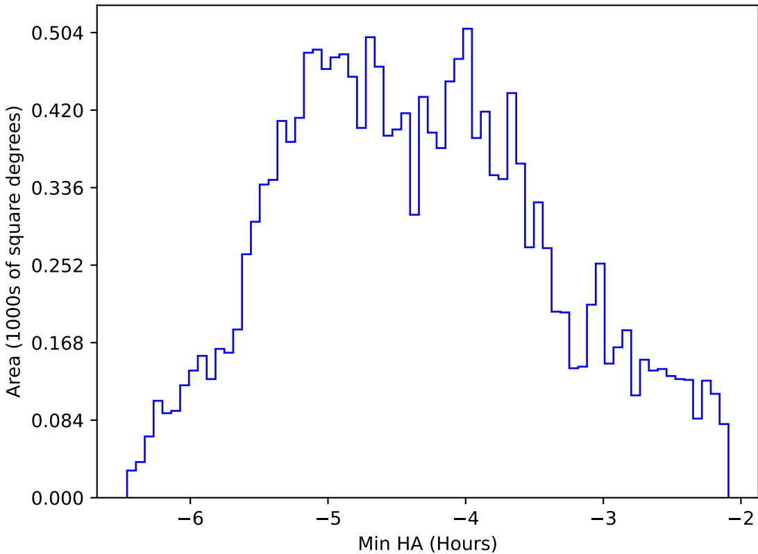
ddf_acor_sf15_lsf20_lsr50_v3.4_10yrs WFD i band: Min HA
