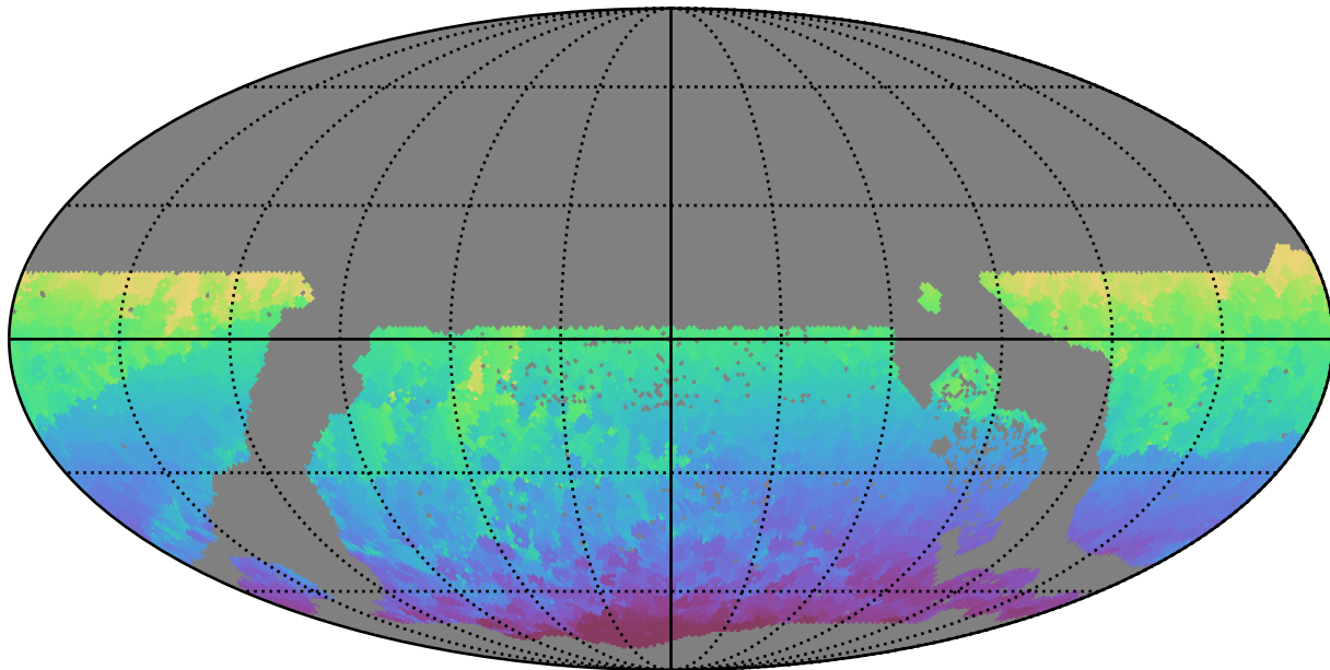
ddf_acor_sf15_lsf20_lsr50_v3.4_10yrs WFD all bands: Min HA
