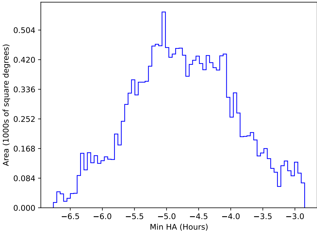
ddf_acor_sf15_lsf20_lsr50_v3.4_10yrs WFD all bands: Min HA
