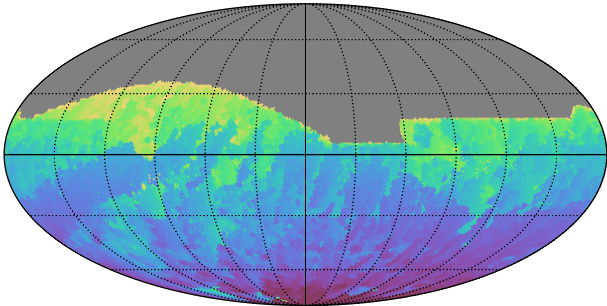
ddf_acor_sf15_lsf20_lsr50_v3.4_10yrs All sky z band: Min HA
