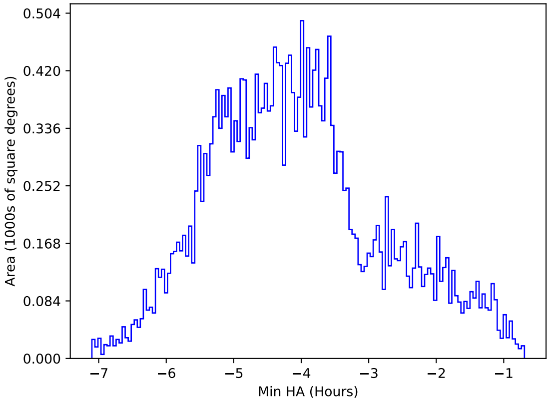
ddf_acor_sf15_lsf20_lsr50_v3.4_10yrs All sky z band: Min HA
