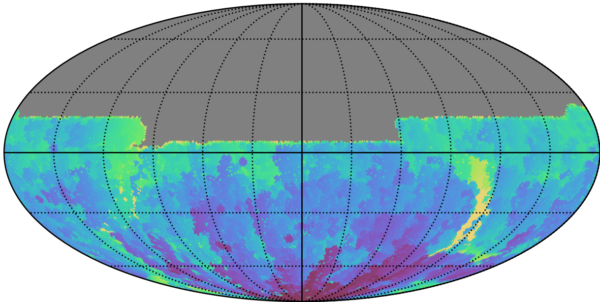
ddf_acor_sf15_lsf20_lsr50_v3.4_10yrs All sky u band: Min HA
