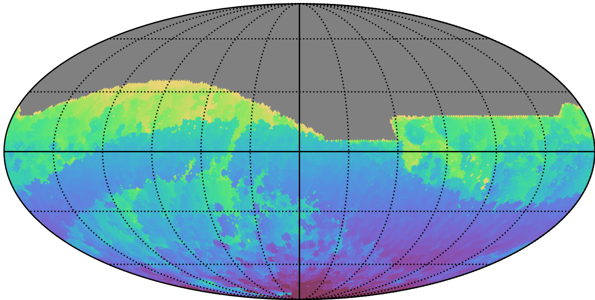
ddf_acor_sf15_lsf20_lsr50_v3.4_10yrs All sky r band: Min HA
