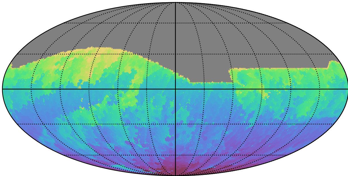
ddf_acor_sf15_lsf20_lsr50_v3.4_10yrs All sky i band: Min HA
