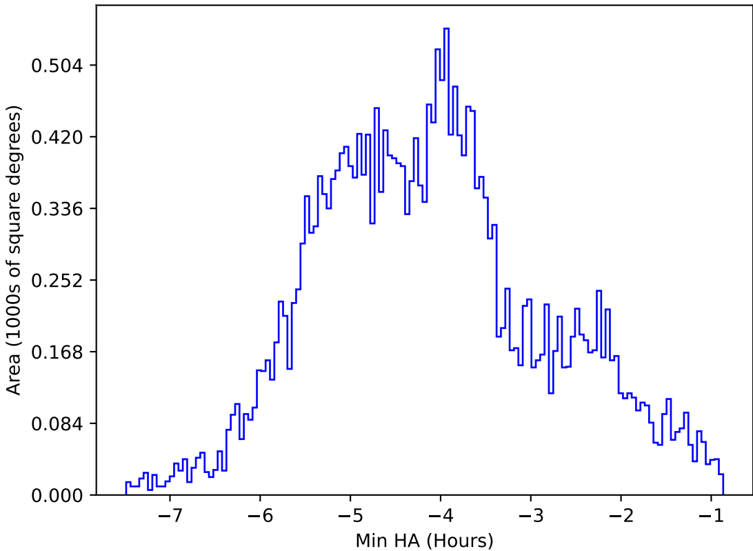
ddf_acor_sf15_lsf20_lsr50_v3.4_10yrs All sky i band: Min HA
