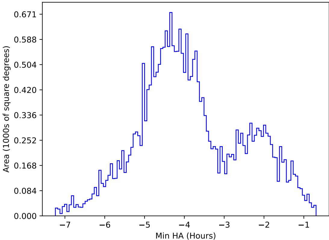
ddf_acor_sf15_lsf20_lsr50_v3.4_10yrs All sky g band: Min HA
