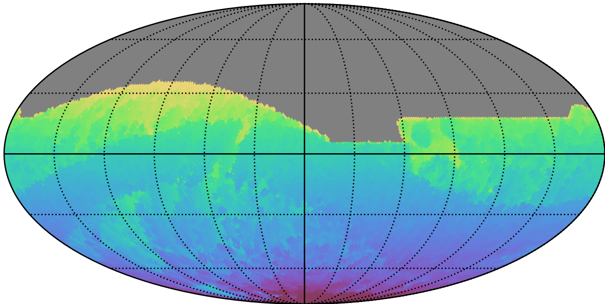
ddf_acor_sf15_lsf20_lsr50_v3.4_10yrs All sky all bands: Min HA
