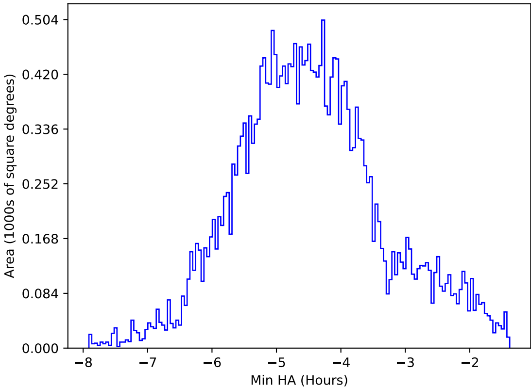
ddf_acor_sf15_lsf20_lsr50_v3.4_10yrs All sky all bands: Min HA
