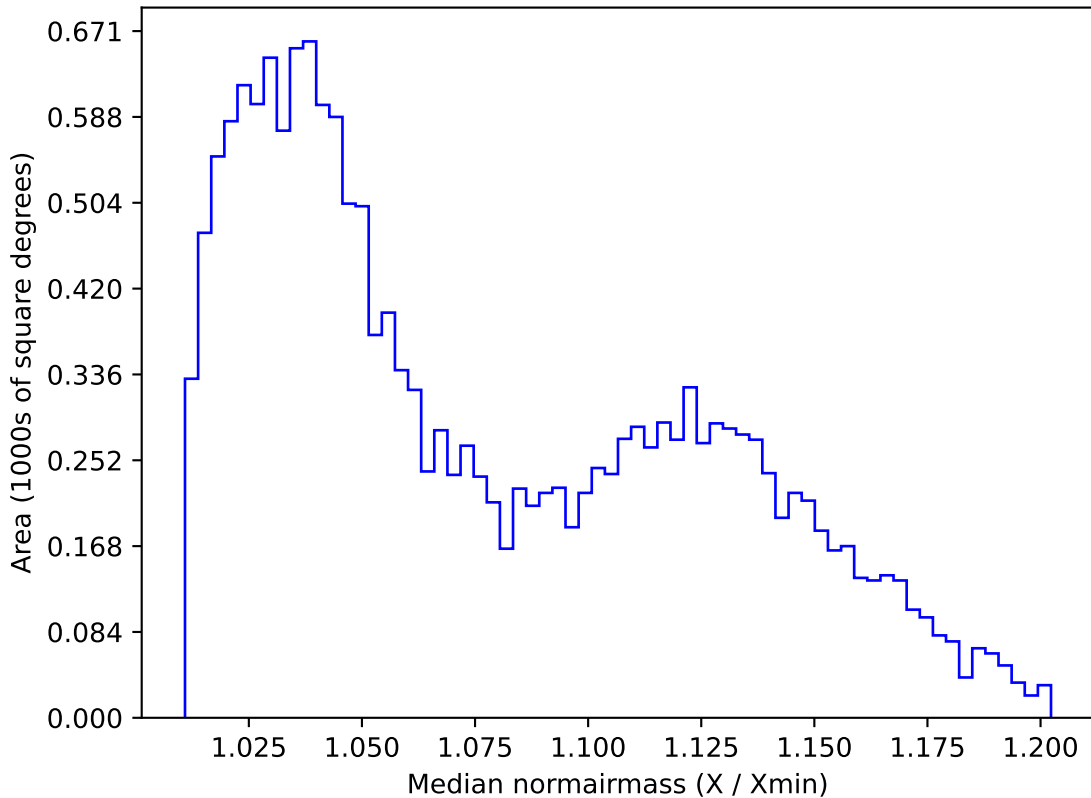
ddf_acor_sf15_lsf20_lsr50_v3.4_10yrs WFD u band: Median normairmass
