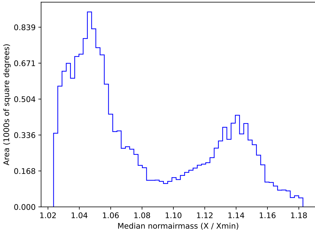
ddf_acor_sf15_lsf20_lsr50_v3.4_10yrs WFD all bands: Median normairmass
