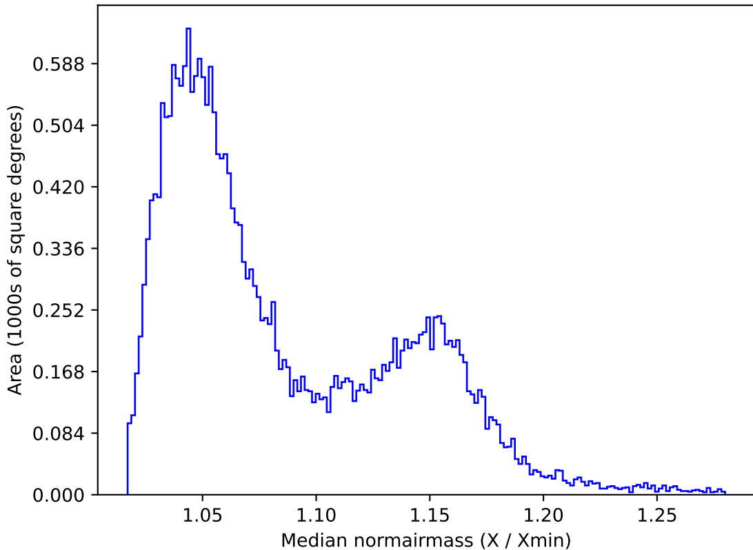
ddf_acor_sf15_lsf20_lsr50_v3.4_10yrs All sky z band: Median normairmass
