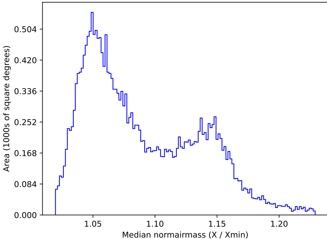
ddf_acor_sf15_lsf20_lsr50_v3.4_10yrs All sky y band: Median normairmass
