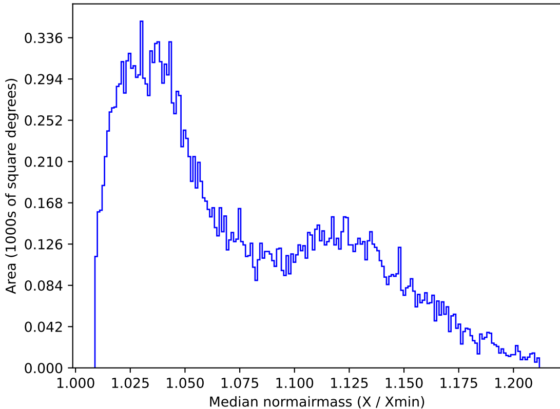
ddf_acor_sf15_lsf20_lsr50_v3.4_10yrs All sky u band: Median normairmass
