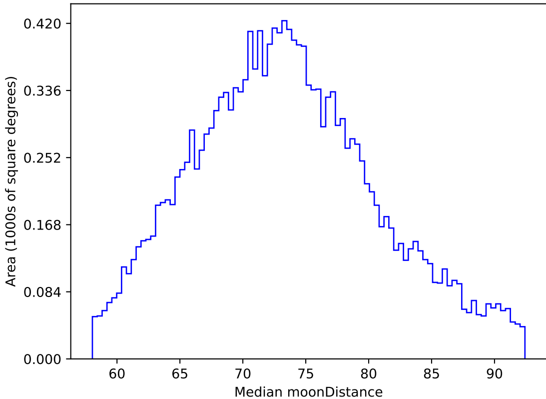
ddf_acor_sf15_lsf20_lsr50_v3.4_10yrs WFD z band: Median moonDistance
