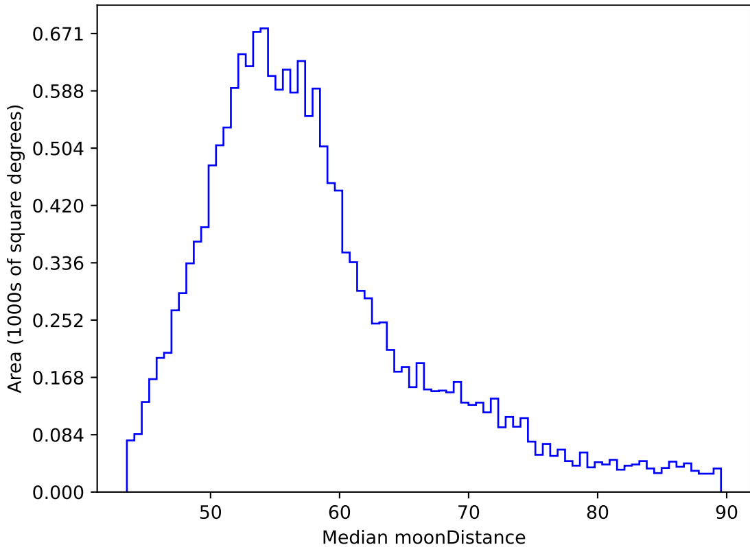
ddf_acor_sf15_lsf20_lsr50_v3.4_10yrs WFD y band: Median moonDistance
