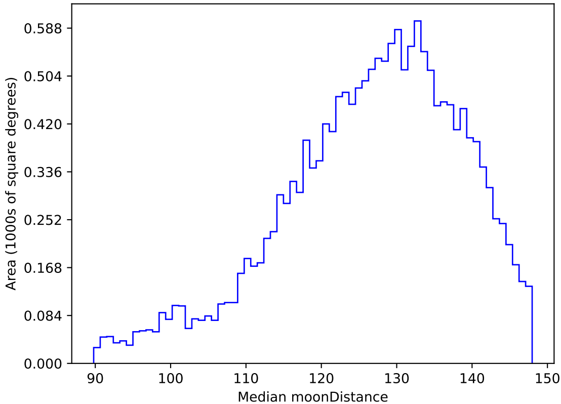
ddf_acor_sf15_lsf20_lsr50_v3.4_10yrs WFD u band: Median moonDistance
