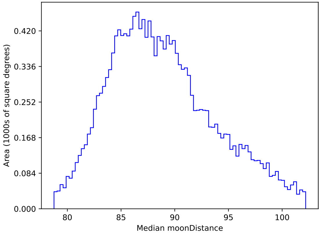
ddf_acor_sf15_lsf20_lsr50_v3.4_10yrs WFD all bands: Median moonDistance
