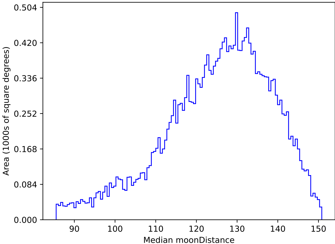
ddf_acor_sf15_lsf20_lsr50_v3.4_10yrs All sky u band: Median moonDistance
