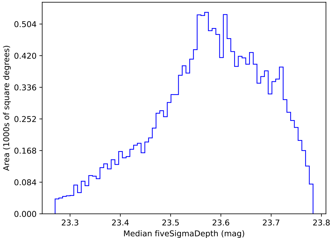
ddf_acor_sf15_lsf20_lsr50_v3.4_10yrs WFD i band: Median fiveSigmaDepth
