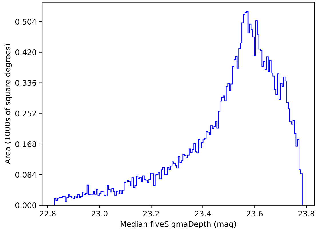
ddf_acor_sf15_lsf20_lsr50_v3.4_10yrs All sky i band: Median fiveSigmaDepth
