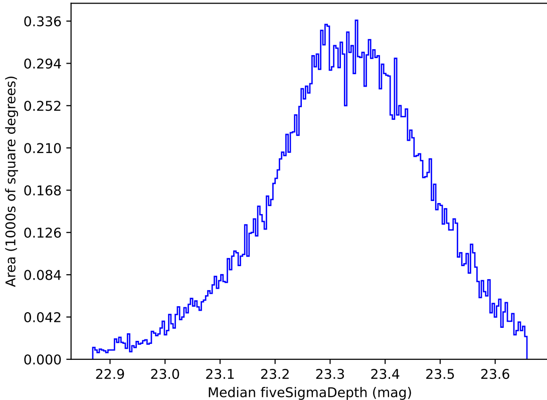
ddf_acor_sf15_lsf20_lsr50_v3.4_10yrs All sky all bands: Median fiveSigmaDepth
